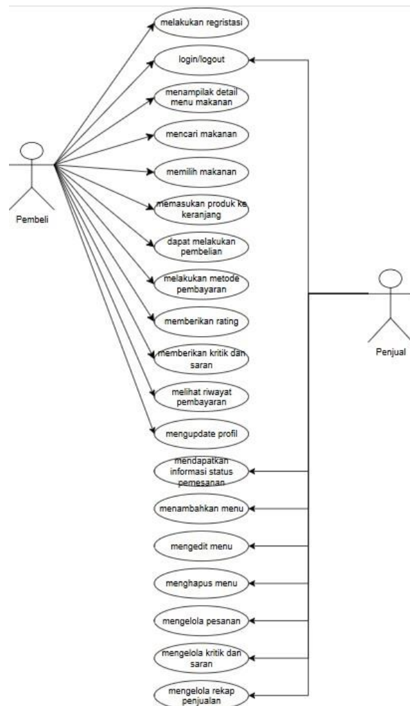
Gambar 2. Diagram Usecase
